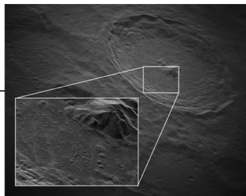
A Synthetic Aperture Radar image of the Moon's Tycho Crater, showing 5-meter resolution detail. Image credit Raytheon.
