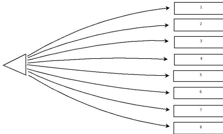
Figure 5: A graphic demonstration of how single beam receivers and beam 1 of the KFPFA can be routed to the VEGAS spectrometers. The routing can be to 1, 2, 3, 4, 5, 6, 7 or 8 different VEGAS spectrometers. This routing is not applicable to a single beam of a dual beam receiver.
